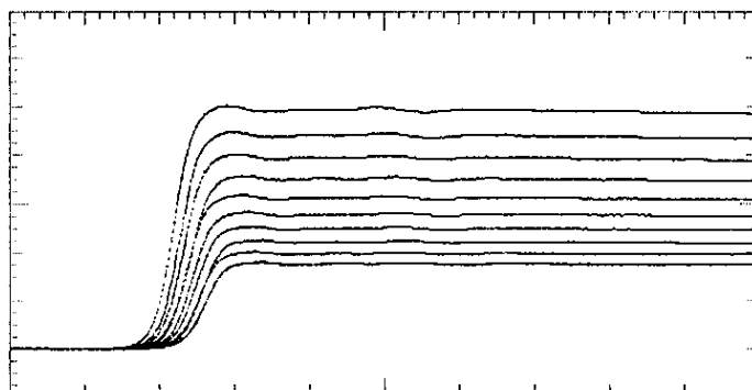
2 V/div and 100 ps/div Adjustable Amplitude in 1 dB steps.
