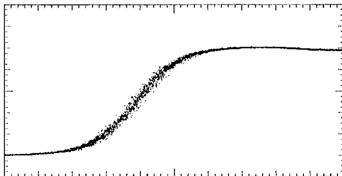
2 V/div and 20 ps/div Leading edge 55 ps Risetime.
