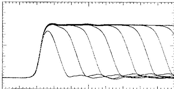
2 V/div and 100 ps/div Adjustable Duration in 2.5 ps steps.
